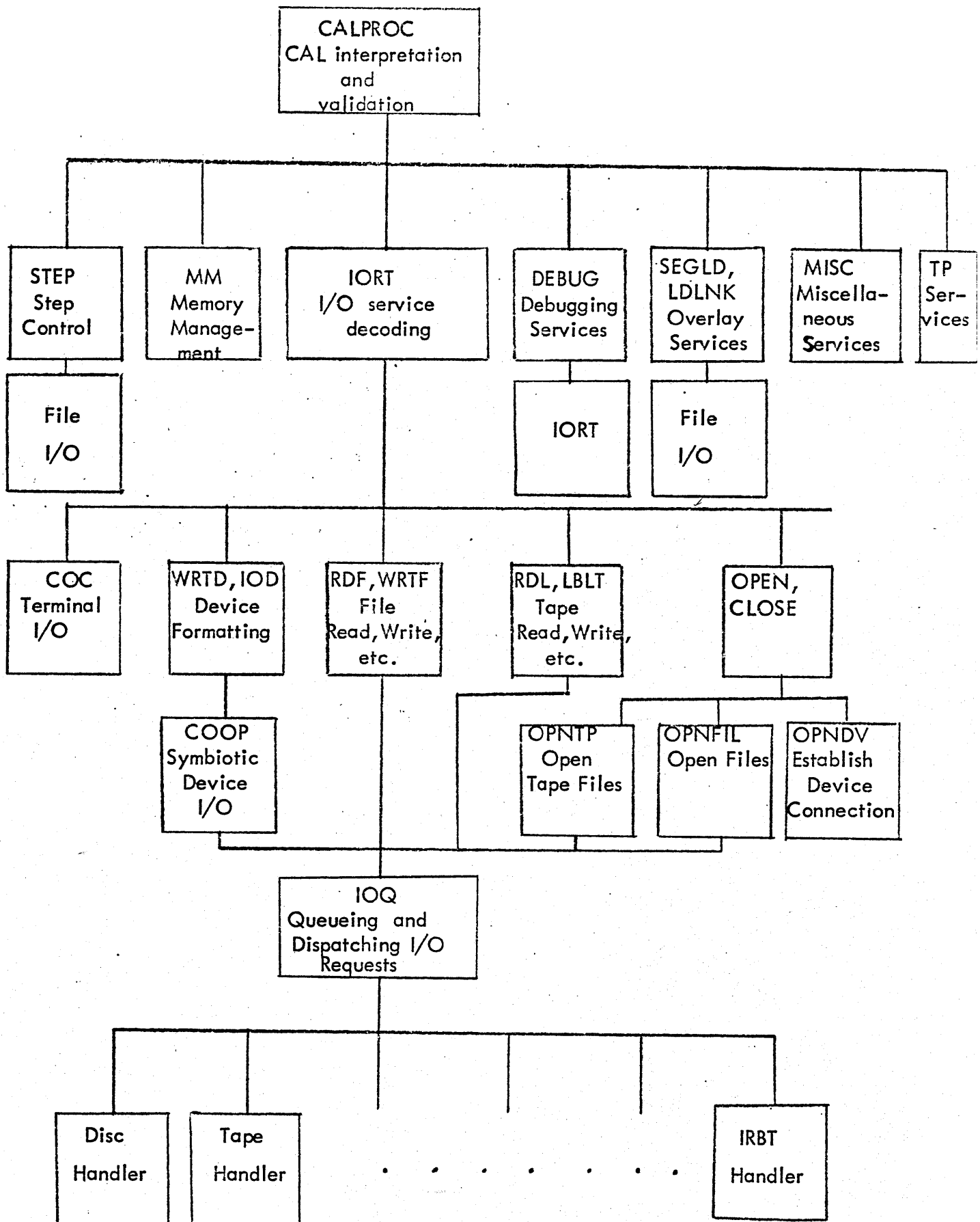
Monitor Service Control Flow
